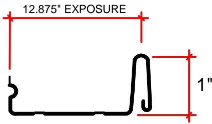
TRI-LOCK 1" SNAP SEAM
