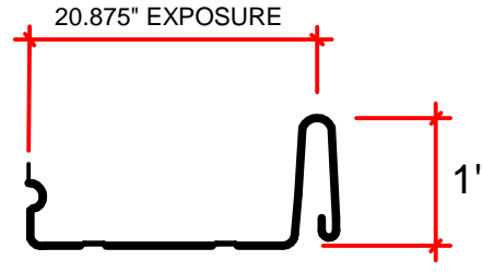
TRI-LOCK 1" SNAP SEAM
