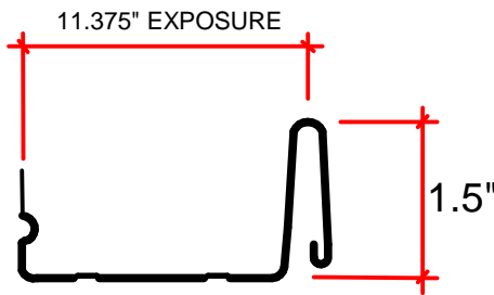
TRI-LOCK 1.5" SNAP SEAM
