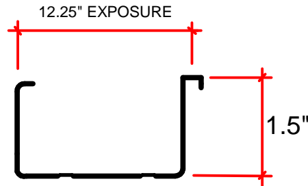
TRI-LOCK 1.5" MECH
