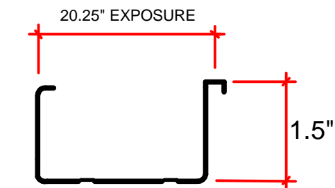
TRI-LOCK 1.5" MECH
