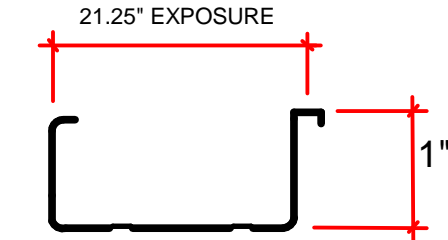
TRI-LOCK 1" MECH
