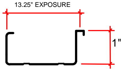
TRI-LOCK 1" MECH
