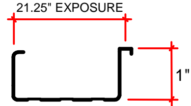
TRI-LOCK 1" MECH
