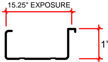
TRI-LOCK 1" MECH
