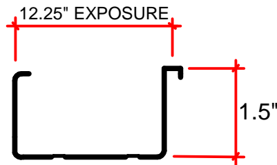
TRI-LOCK 1.5" MECH
