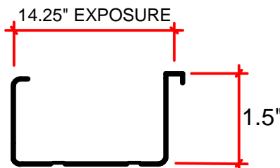
TRI-LOCK 1.5" MECH
