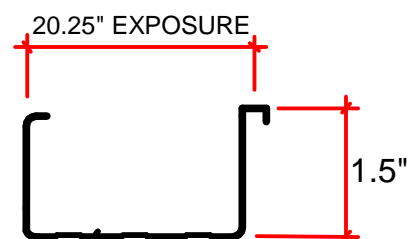
TRI-LOCK 1.5" MECH
